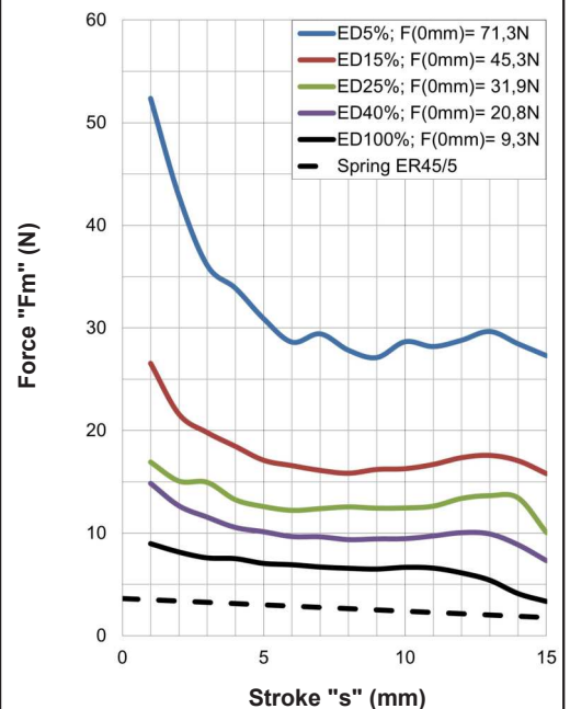
Force-stroke curve
