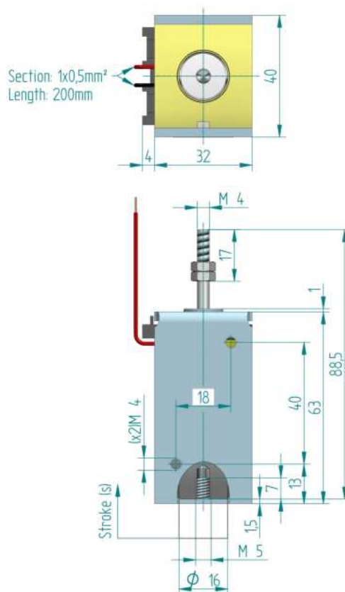
Solenoid locked (s=0mm position)
