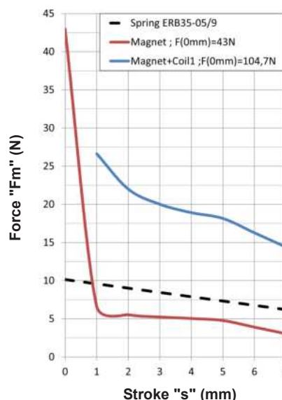
Force-stroke curve(F-S)
