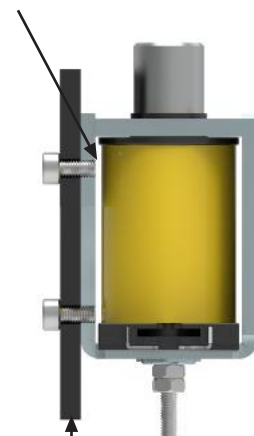
Assembly panel
